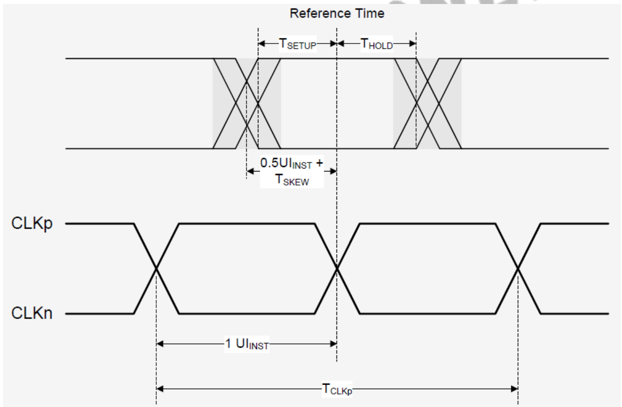
Figure 6-41 MIPI DPHY Timing
