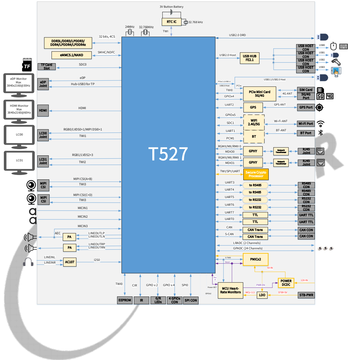
Figure 4-2 Typical Application
